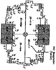
DETAIL BUILDING 20 (NOT TO SCALE)
